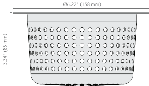
3.3" Debris Strainer Basket
