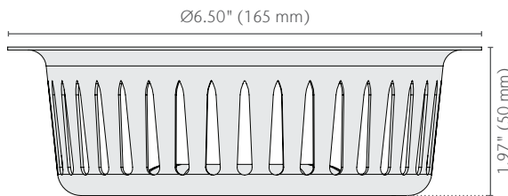
2.0" Debris Strainer Basket
